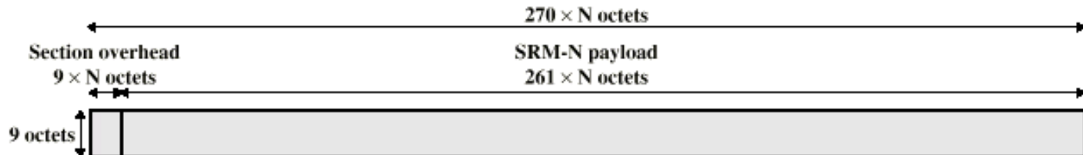
(b) STM-N frame format
