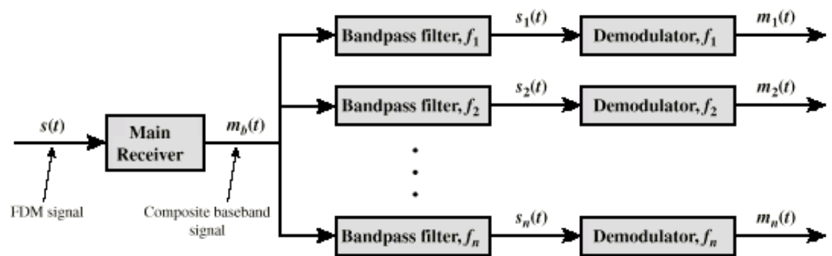
(c) Receiver
