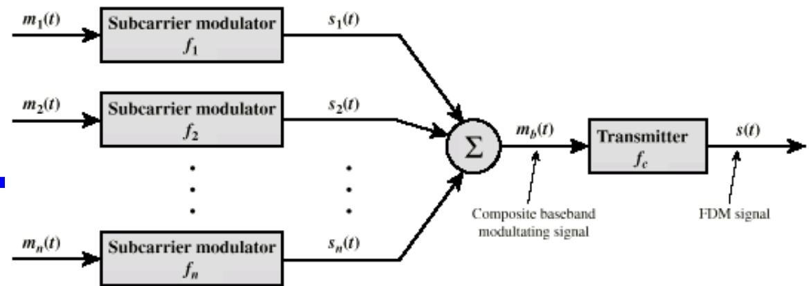
(a) Transmitter
