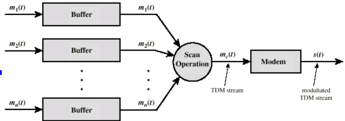
(a) Transmitter
